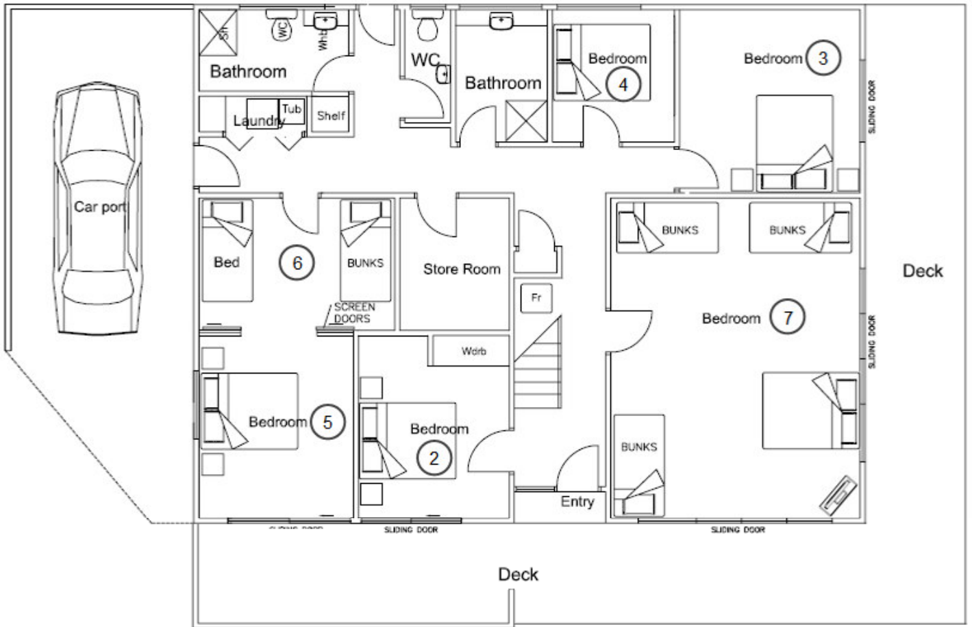
LOWER FLOOR
